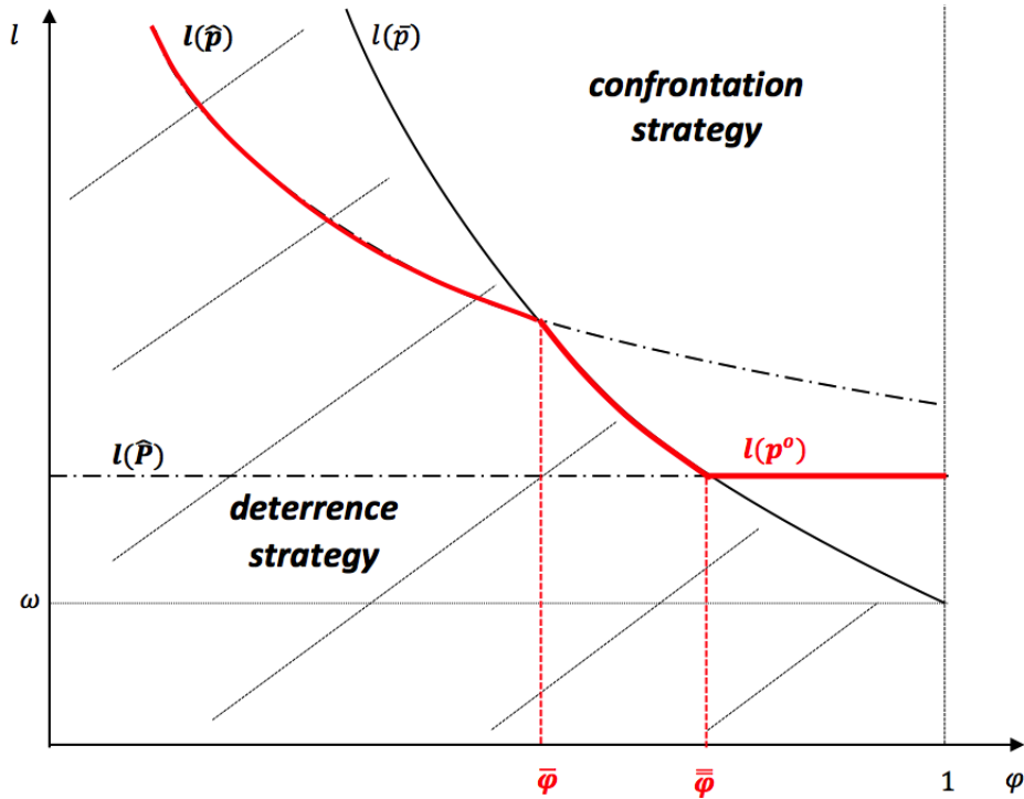
Figure 2: Equilibrium outcomes with endogenous l : l(P^*) > 1 .
